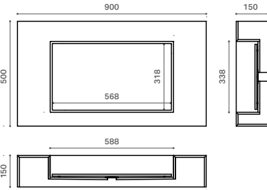
90×50 cm scarico nascosto/concealed drainage
