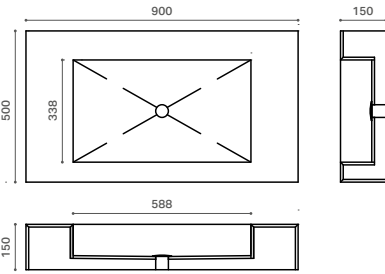
90×50 cm scarico a vista/visible drainage
